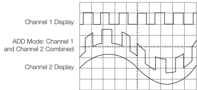
Figure 37. Adding channels.
