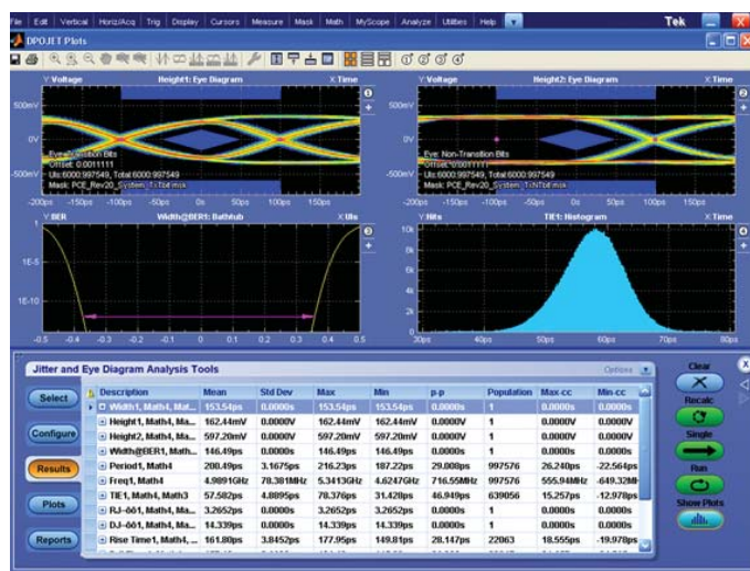
Figure 53. Analysis software packages are specifically designed to meet jitter and eye measurement needs of today's high-speed digital designers.
