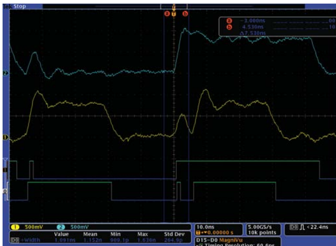
Figure 51. The MSO provides 16 integrated digital channels, enabling the ability to view and analyze time-correlated analog and digital signals. A high speed timing acquisition provides more resolution to reveal narrow events such as glitches.
