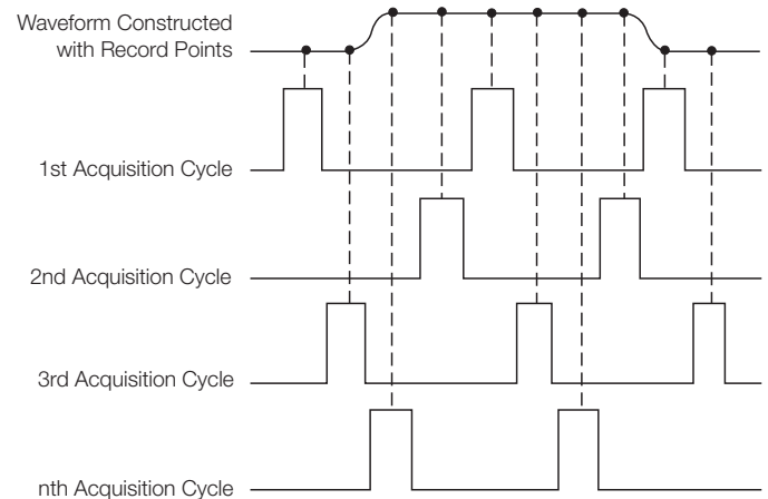
Figure 29. Some oscilloscopes use equivalent-time sampling to capture and display very fast, repetitive signals.
