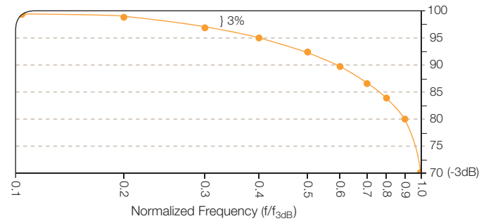
Figure 43. Oscilloscope bandwidth is the frequency at which a sinusoidal input signal is attenuated to 70.7% of the signal's true amplitude, known as the -3 dB point.
