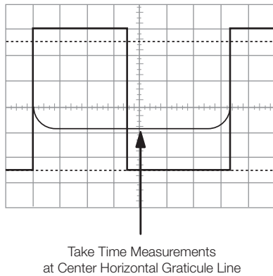
Figure 67. Measure time on the center horizontal graticule line.
