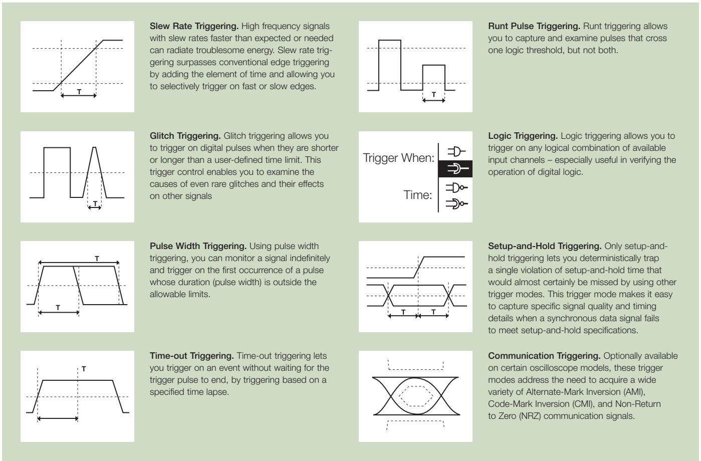
Figure 33. Common trigger types.
