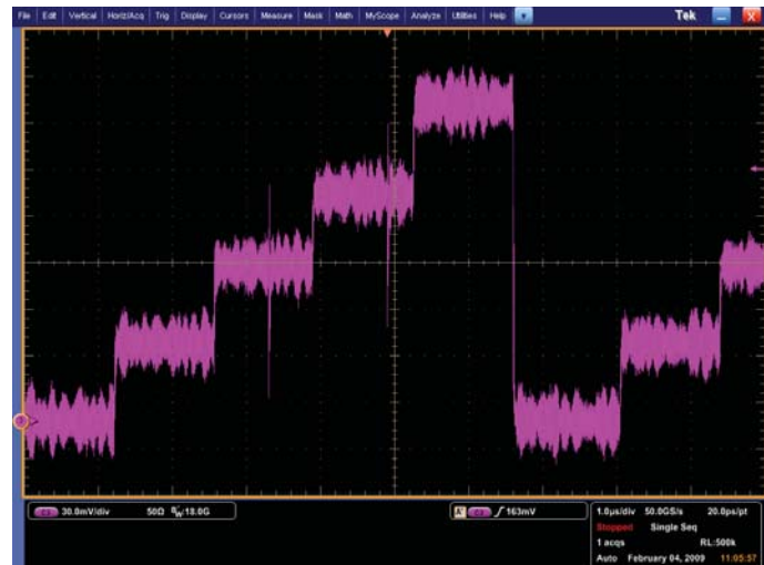
Figure 23. Peak detect mode enables the oscilloscope to capture extremely brief transient anomalies.
