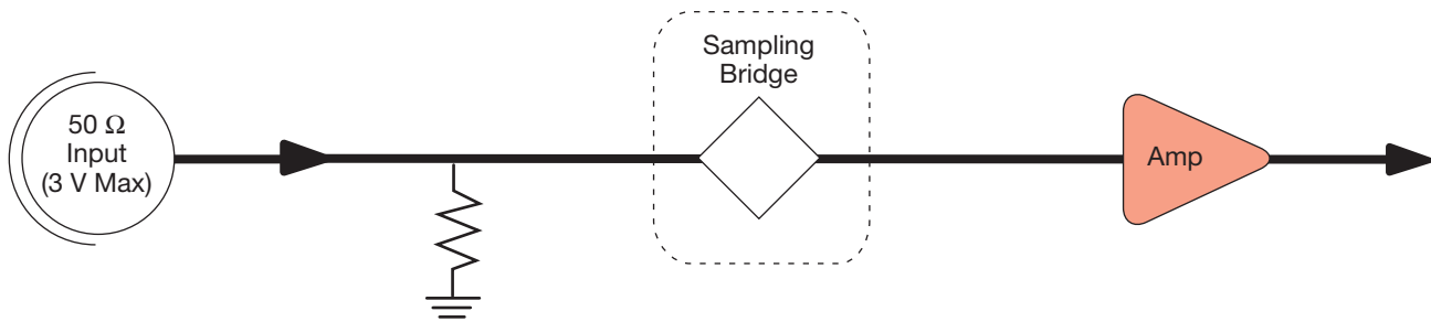
Figure 17. The architecture of a digital sampling oscilloscope.
