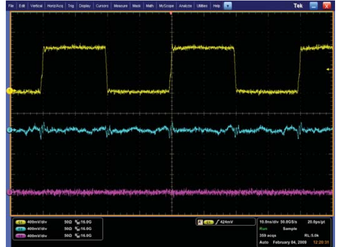
Figure 41 Differential probes can separate common-mode noise from the signal content of interest in today's fast, low-voltage applications - especially important as digital signals continue to fall below typical noise thresholds found in integrated circuits.
