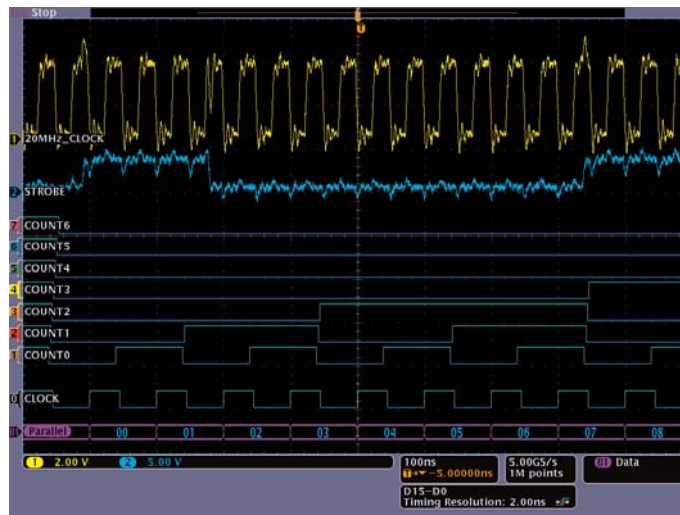
Figure 16. The MSO provides 16 integrated digital channels, enabling the ability to view and analyze time-correlated analog and digital signals.
