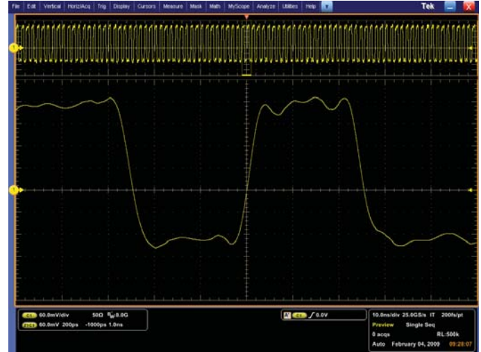
Figure 45. Rise time characterization of a high-speed digital signal.
