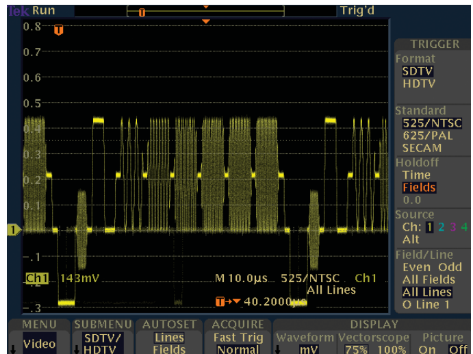
Figure 57. Video application modules make the oscilloscope a fast, tell-all tool for video troubleshooting.
