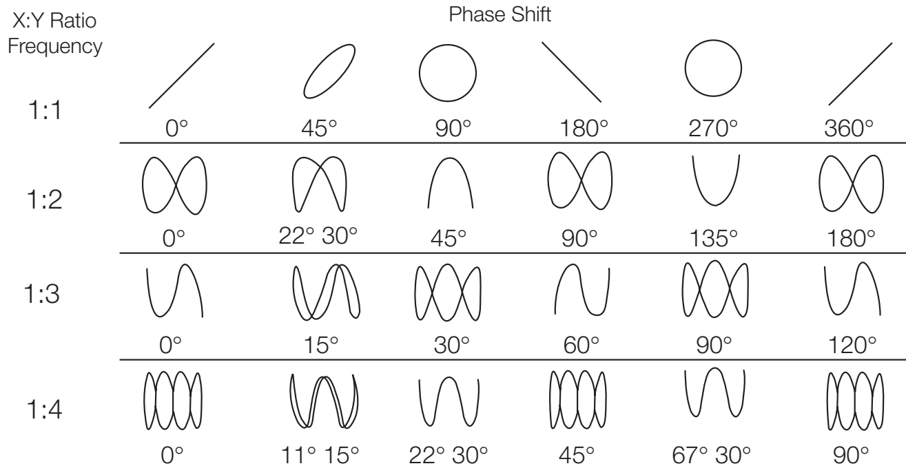
Figure 69. Lissajous patterns.
