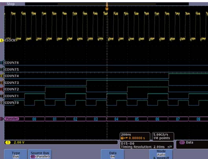
Figure 55. Automatically trigger, decode, and search on clocked or unclocked parallel bus data.
