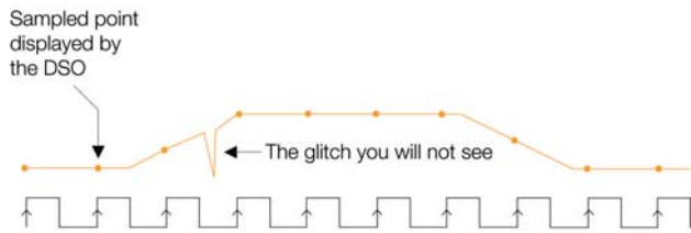
Figure 22. Sample rate varies with time base settings - the slower the time based setting, the slower the sample rate. Some digital oscilloscopes provide peak detect mode to capture fast transients at slow sweep speeds.
