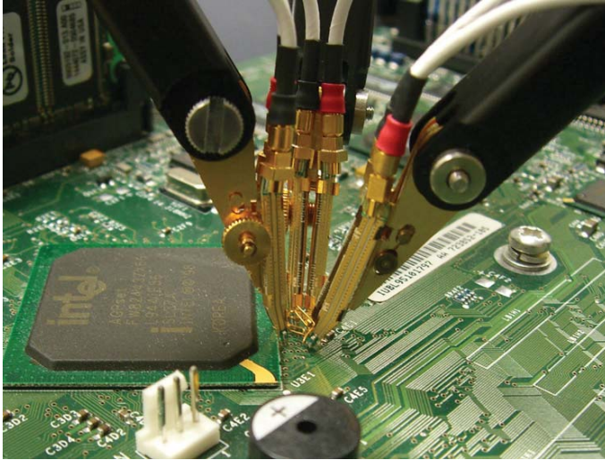
Figure 40. High-performance probes are critical when measuring the fast clocks and edges found in today's computer buses and data transmission lines.
