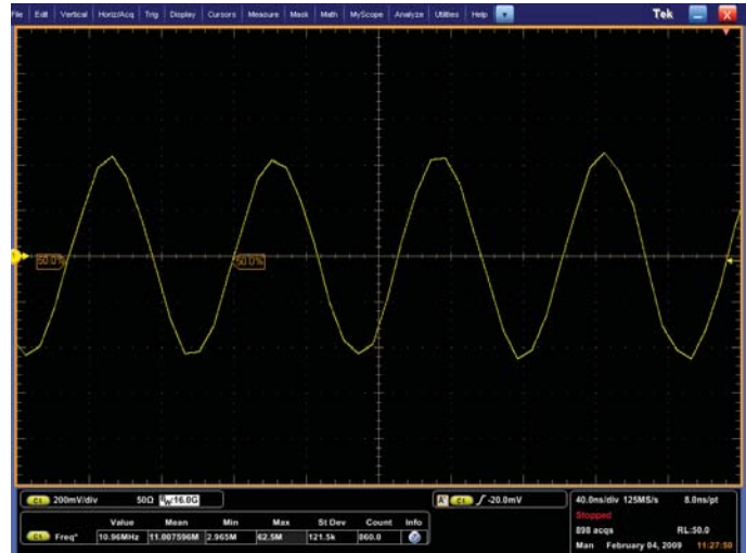
Figure 27. Undersampling of a 100 MHz sine wave introduces aliasing effects.
