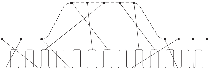
Figure 30. In random equivalent-time sampling, the sampling clock runs asynchronously with the input signal and the trigger.
