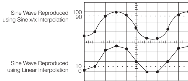
Figure 28. Linear and sin x/x interpolation.
