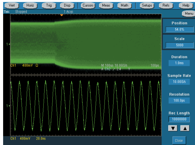
Figure 50. Capturing the high frequency detail of this modulated 85 MHz carrier requires high resolution sampling (100 ps). Seeing the signal's complete modulation envelope requires a long time duration (1 ms). Using long record length (10 MB), the oscilloscope can display both.
