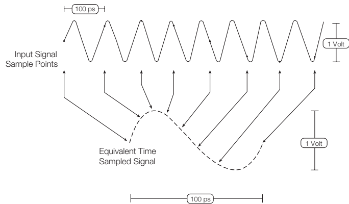
Figure 24. Basic sampling, showing sample points are connected by interpolation to produce a continuous waveform.
