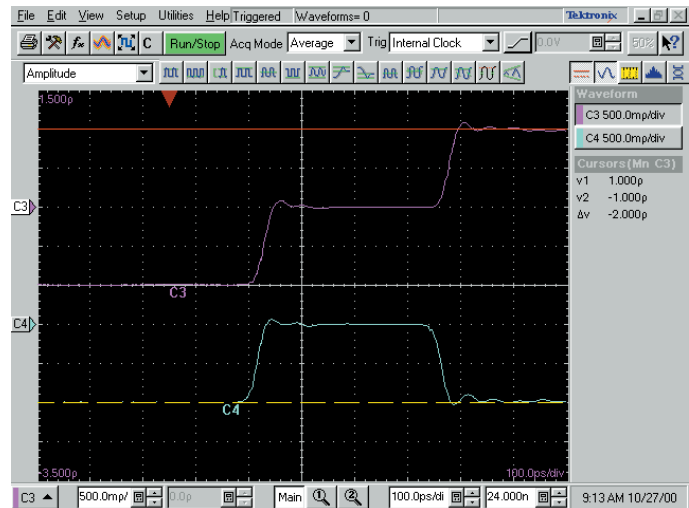
Figure 18. Time domain reflectometry (TDR) display from a digital sampling oscilloscope.
