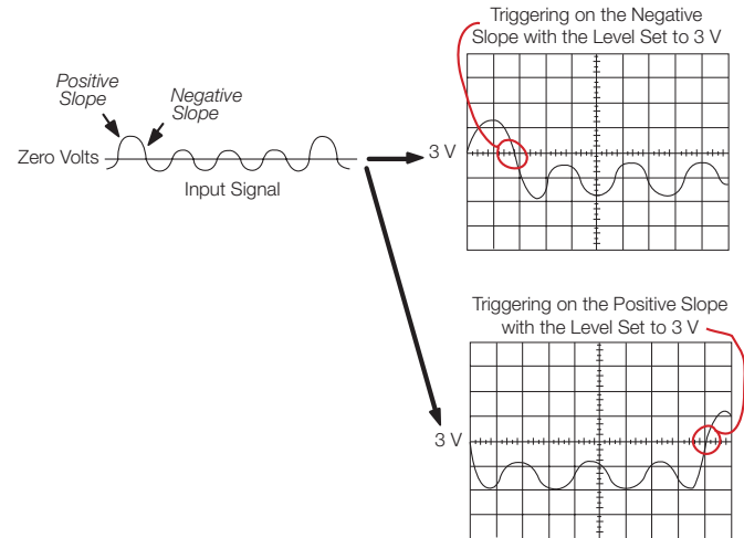
Figure 34. Positive and negative slope triggering.
