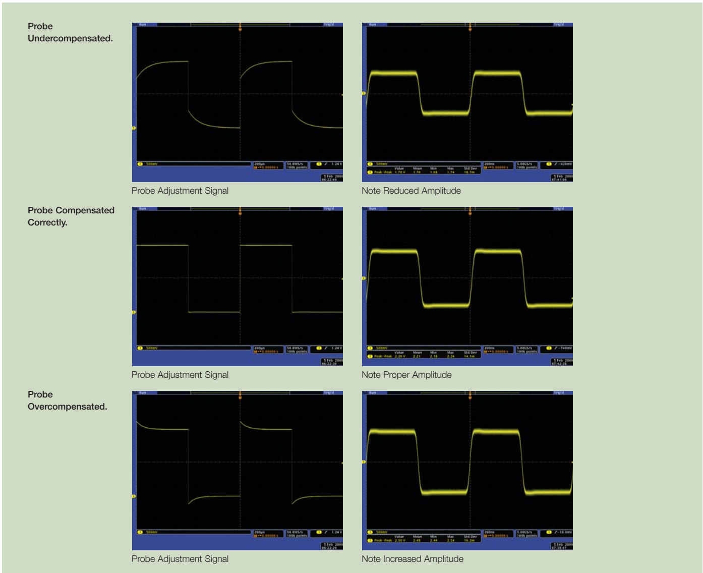
Figure 64. The effects of improper probe compensation.
