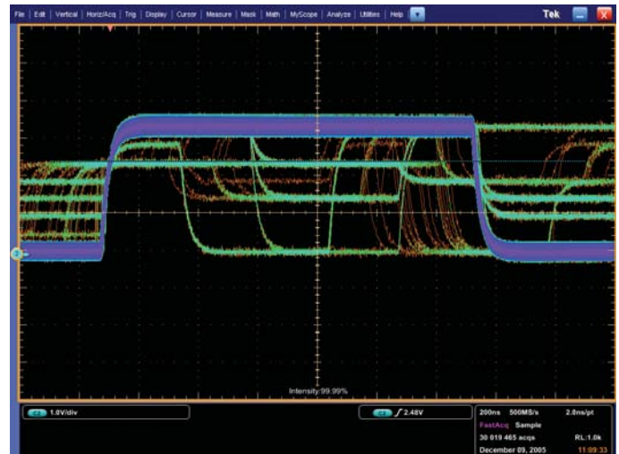
Figure 49. A DPO enables a superior level of insight into signal behavior by delivering vastly greater waveform capture rates and three-dimensional display, making it the best general-purpose design and troubleshooting tool for a wide range of applications.
