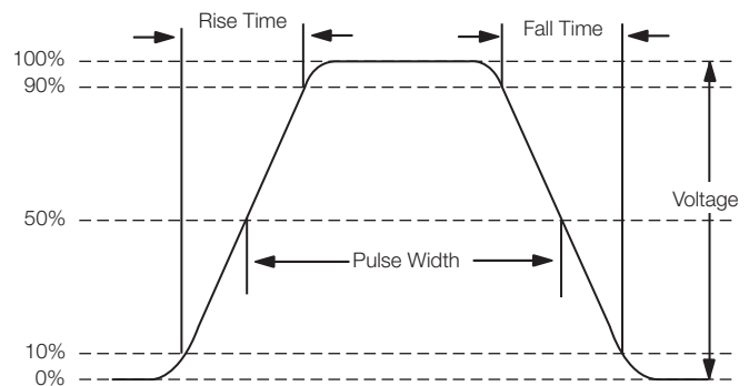
Figure 68. Rise time and pulse width measurement points.
