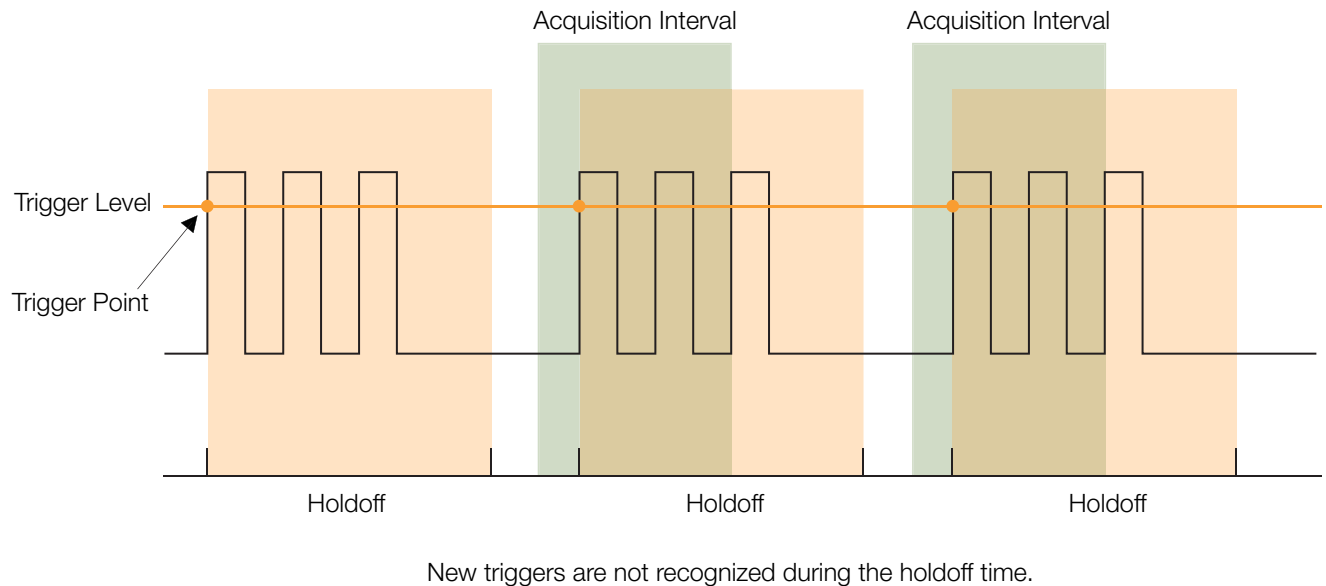
Figure 35. Trigger holdoff.
