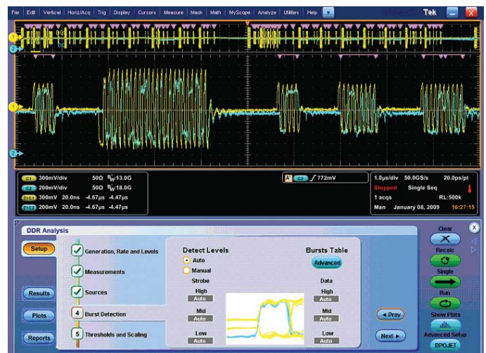
Figure 56. Advanced DDR analysis tools automate complex memory tasks like separating read/write bursts and performing JEDEC measurements.
