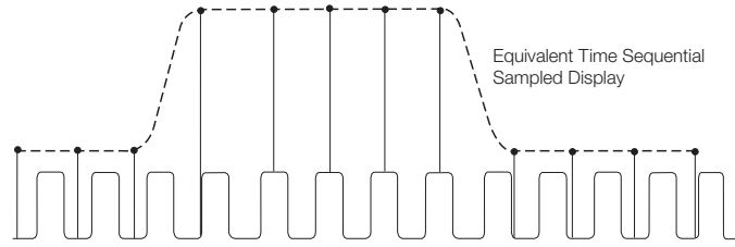
Figure 31. In sequential equivalent-time sampling, the single sample is taken for each recognized trigger after a time delay which is incremented after each cycle.
