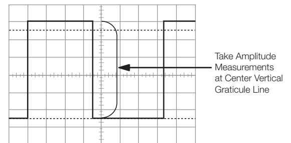
Figure 65. Voltage peak ( V_p ) and peak-to-peak voltage ( V_{p-p} )
