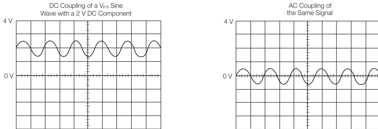
Figure 20. AC and DC input coupling.
